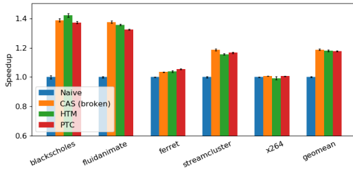
Fig. 10: PARSEC suite with 10 cores.
