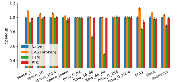
Fig. 11: Micro-benchmarks with 1 core.
