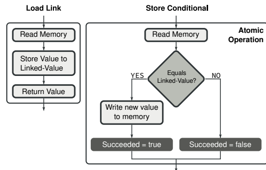
Fig. 3: An example of how compare-and-swap semantics can be used to approximate load-link/store-conditional semantics.
