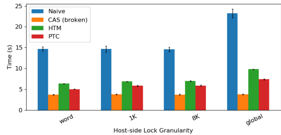
Fig. 13: Micro-benchmark space_1024 in 8-core configuration with varying host-side lock granularity.
